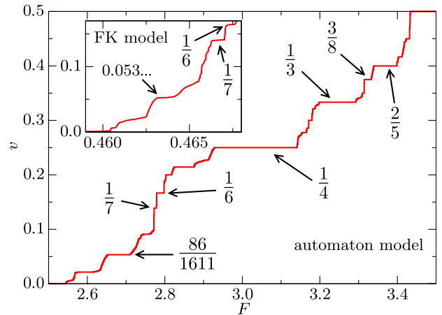
FIG. 1 (color online). The activity staircase, velocity v vs drive F , for the quasiperiodic automaton of size L_x \times L_y = 169 \times 153 with pinning given by the rational approximants (70/169, 112/153) to (\sqrt{2} - 1, \sqrt{3} - 1) . Fractions with small denominators generally have the widest mode-locked steps, but the step at 86/1611 is an anomalous step which does not fit this pattern. Inset: results for the FK model, Eq. (2), with h = 10 and the same size and quasiperiodic pinning; an anomalous step with similar v \approx 0.053 is seen.
