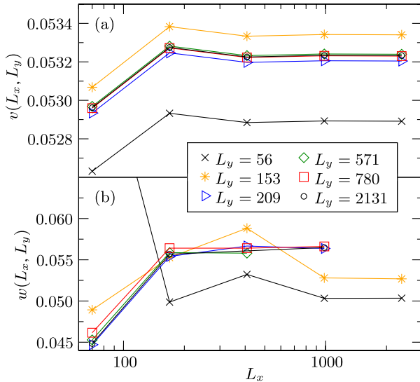
FIG. 2 (color online). The size dependence of (a) activity v(L_x, L_y) , and (b) width, w(L_x, L_y) , of the anomalous step. Each curve is for fixed L_y . The convergence of v and w as a function of system size strongly suggests that there is a well-defined activity \hat{v} and step width \hat{w} in the limit (L_x, L_y) \rightarrow (\infty, \infty) ; we conjecture that \hat{v} \notin \mathbb{Q} , Eq. (9), and \hat{w} \neq 0 .
