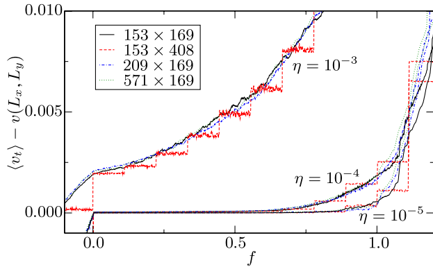
FIG. 3 (color online). The effect of thermal noise on the anomalous step for dimensionless noise values \eta = 10^{-5} , 10^{-4} , 10^{-3} for system sizes defined in the key. The horizontal axis is the scaled force f which is linear in F with each zero-temperature step starting at f = 0 and ending at f = 1 . For easier comparison, the zero-temperature activity v(L_x, L_y) has been subtracted. For each value of noise, there is similar rounding of the plateau for all system sizes.
